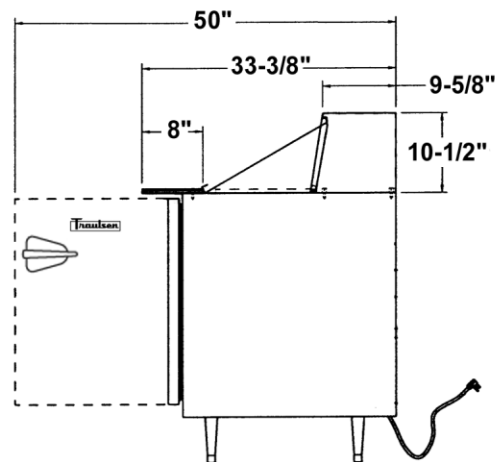
Section - UPT4818
