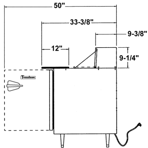
Section - UPT4812
