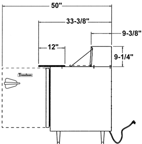
Section - UPT488
