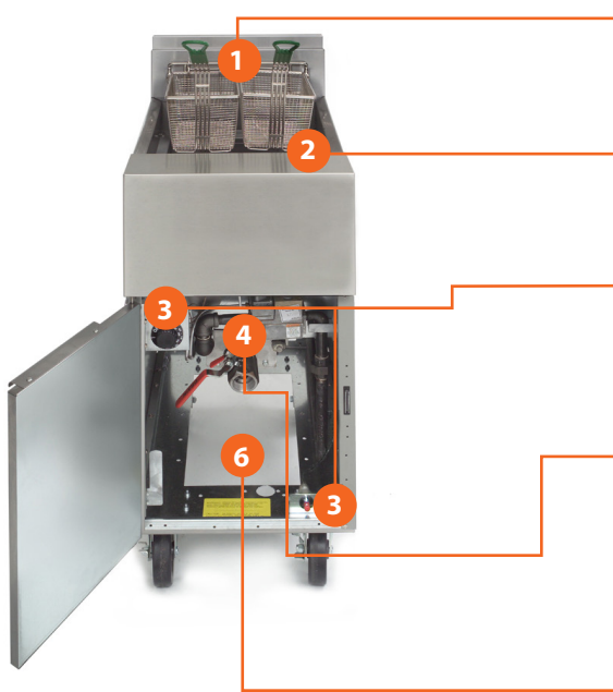
GF14 fryer shown with optional and Piezo ignitor
